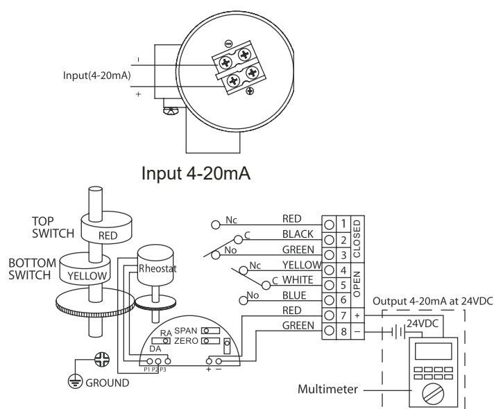
Output 4-20mA &amp; Limit Switch 2-SPDT
