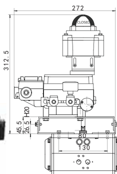
ALP-1000RDd53+ALS300M2T (2-SPDT, 4-20mA Position Transmitter)
