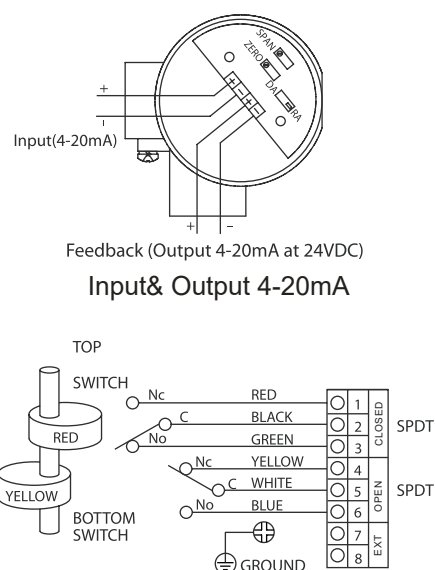
Limit Switch 2-SPDT
