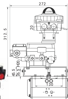
ALP-1000RDd53+ALS400M2T (2-SPDT, 4-20mA Position Transmitter)
