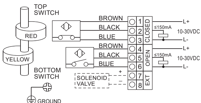
ALS200/206/300/400/500/600PA23 PNP NO (3-Wire) Inductive Sensors
