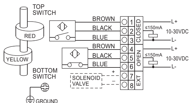
ALS200/206/300/400/500/600PA23 PNP NC (3-Wire) Inductive Sensors
