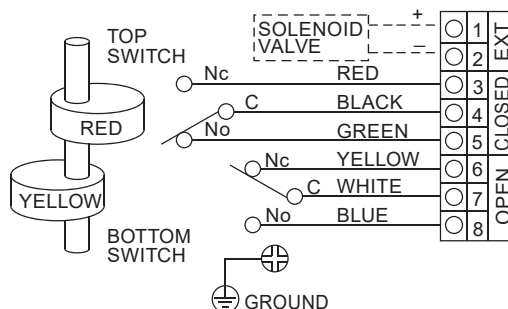
ALS-500/600M2 2SPDT Mechanical Switches Wiring
