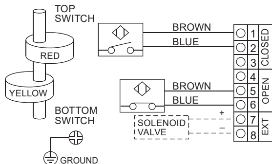
ALS200/206/300/400/500/600PP22/PA22 NC (2-Wire) Inductive Sensors
