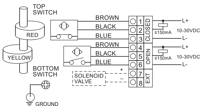
ALS200/206/300/400/500/600PA23 NPN NO (3-Wire) Inductive Sensors
