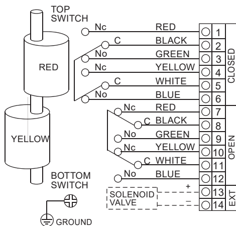
ALS-206/300/400/500/600M5 2DPDT Mechanical Switches Wiring
