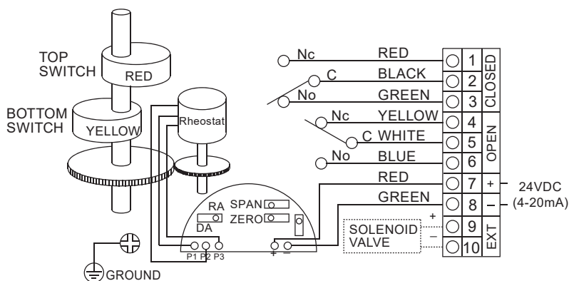
ALS-300/400M2T 2SPDT Mechanical Switches Wiring
