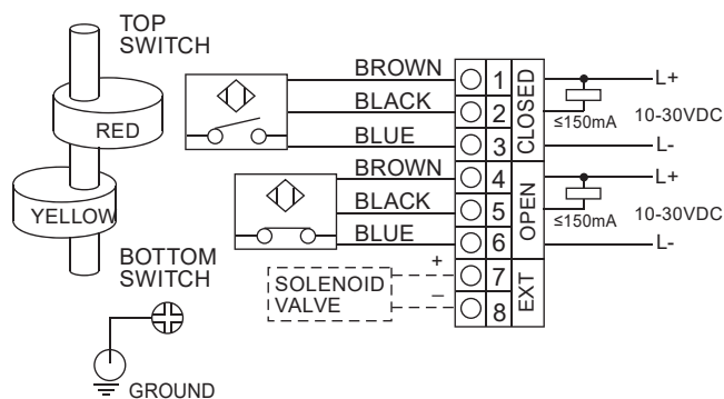
ALS200/206/300/400/500/600PA23 NPN NC (3-Wire) Inductive Sensors
