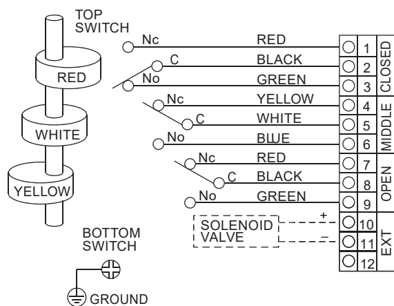
ALS-206/300/400/500/600M3 3SPDT Mechanical Switches Wiring
