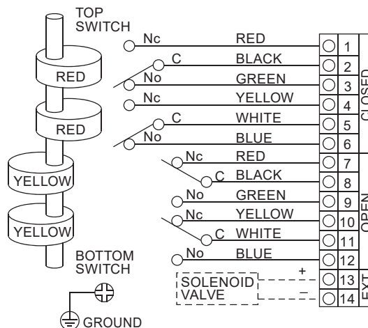
ALS-206/300/400/500/600M4 4SPDT Mechanical Switches Wiring
