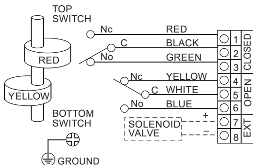
ALS-200/206/300/400M2 2SPDT Mechanical Switches Wiring
