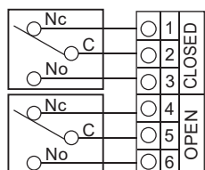
ALS-105 2SPDT Mechanical Switches Wiring
