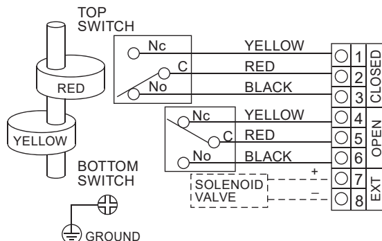
ALS200/206/300/400/500/600QA23 NC (3-Wire) Magnet Sensors
